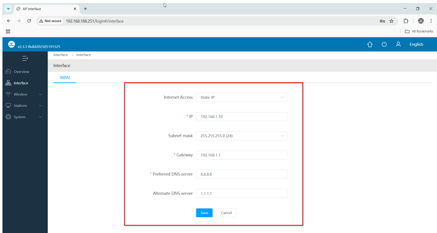
Fig 2.5 Port Setting DNS of AIR-AP01200
