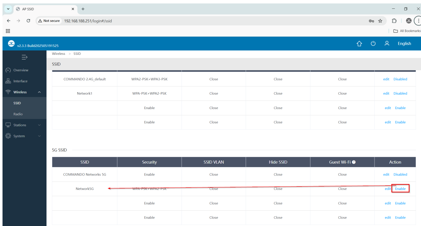
Fig 3.1.17 Setting VAP New SSID in 5G band of AIR-AP01200
