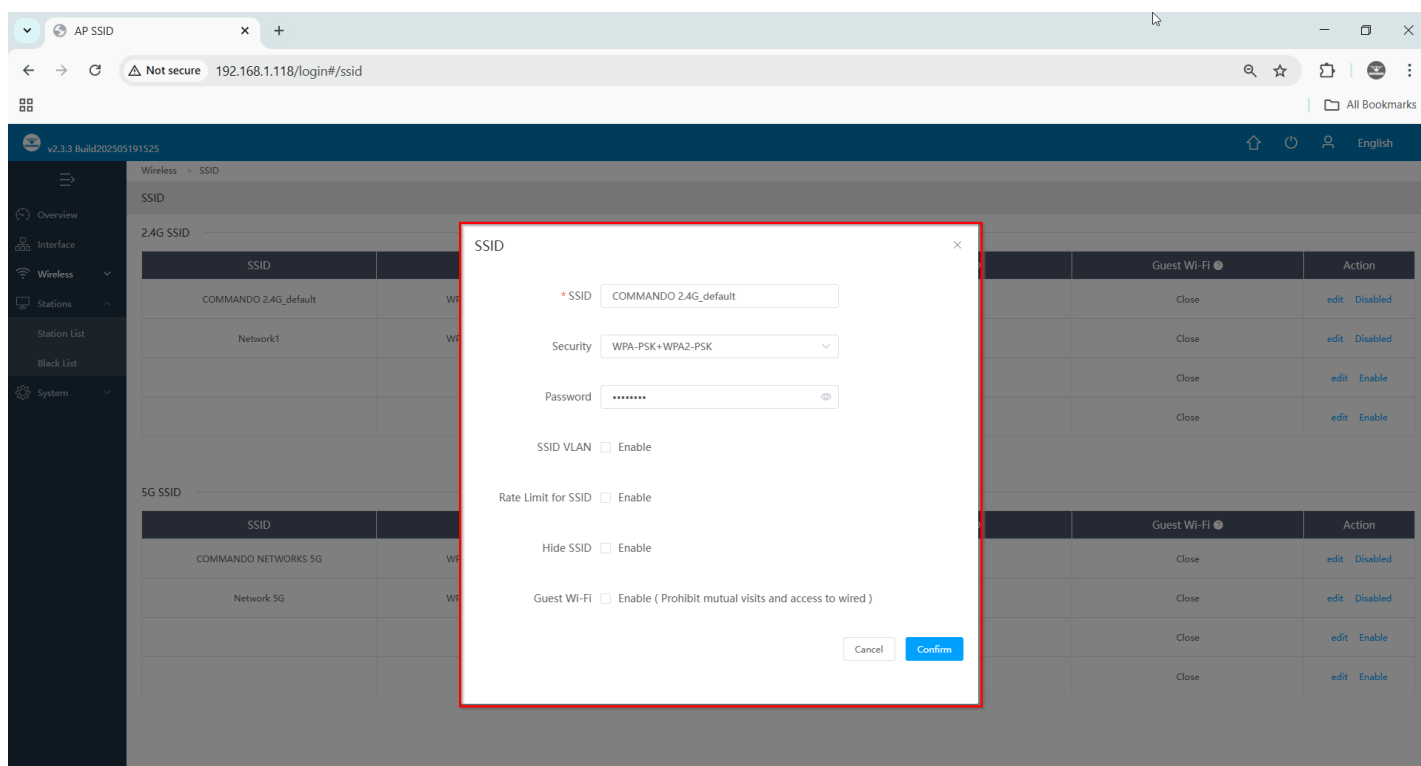
Fig 3.1.3 SSID Setting of AIR-AP01200
